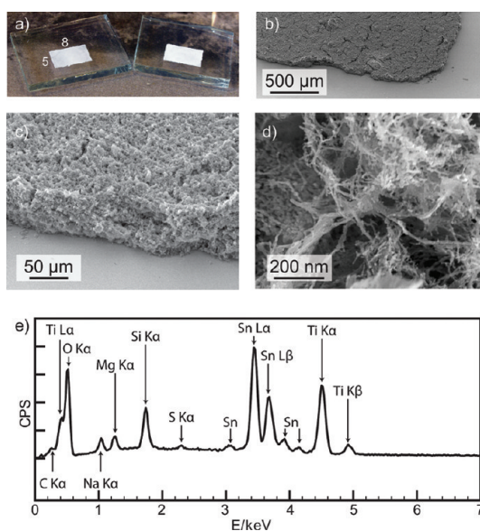
Figure 3. Films cast from a crushed hollow \text{TiO}_2 nanotube dispersion in ethanol. (a) Photographs of a 15 (left) and 25 \mu\text{m} (right) thick films. Film dimensions are 5 \times 8\text{ mm} . (b) Tilted SEM image shows that the \text{TiO}_2 film ( ca. 50 \mu\text{m} thick) with only a few cracks has formed on the substrate. (c) Larger magnification shows the edge of the film. The film consists of granules of micrometer dimensions. (d) High magnification image shows that the granules are formed of networks of \text{TiO}_2 tubes. (e) Energy dispersive X-ray spectrum shows that there is only very little carbon in the film and the \text{TiO}_2 content is high. Other peaks originate from the FTO glass.
